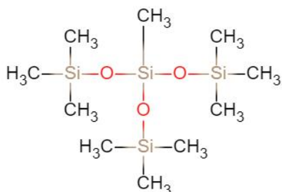
Structural formula
